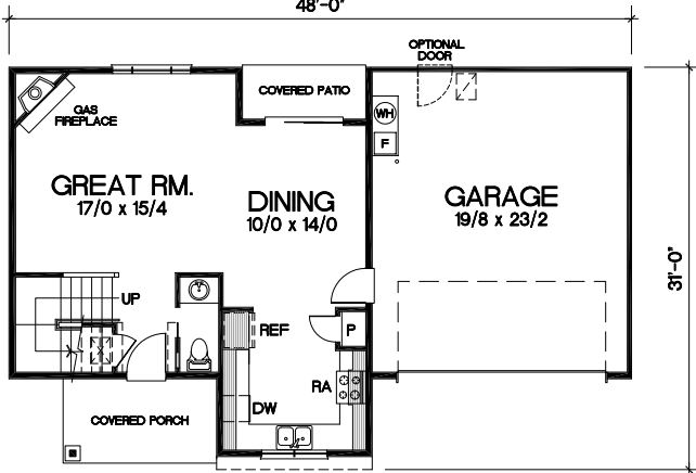
MAIN FLOOR (655 SQ. FT.) 31'-0"
